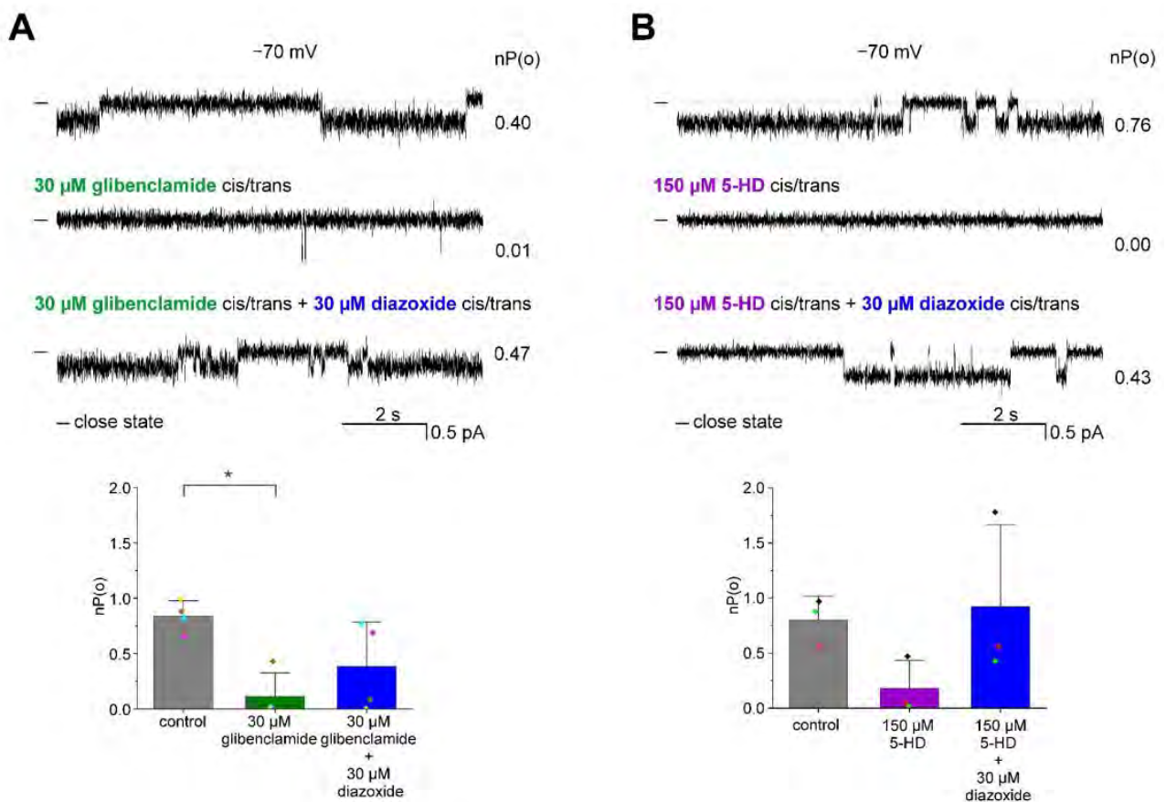
Figure 6. Inhibition of ROMK2 channel activity by glibenclamide and 5-HD. (A) Glibenclamide inhibits the activity of the ROMK2 channel. Top panel: Representative single-channel recordings at -70 mV under control conditions, in the presence of 30 \mu\text{M} glibenclamide followed by the addition of 30 \mu\text{M} diazoxide. Lower panel: Channel open probability, nP(o) , under control conditions, in the presence of 30 \mu\text{M} glibenclamide and after the addition of 30 \mu\text{M} diazoxide ( n = 4 ). (B) 5-HD blocks the activity of the ROMK2 channel. Top panel: Representative single channel recordings at -70 mV under control conditions, in the presence of 150 \mu\text{M} 5-HD and after the addition of 30 \mu\text{M} diazoxide. Lower panel: Channel open probability, nP(o) , in control conditions, in the presence of 150 \mu\text{M} 5-HD, or 150 \mu\text{M} 5-HD and 30 \mu\text{M} diazoxide ( n = 3 ). “-” indicates a closed state of the channel. The results related to channel open probability are presented as means \pm SD. * p < 0.05 .
